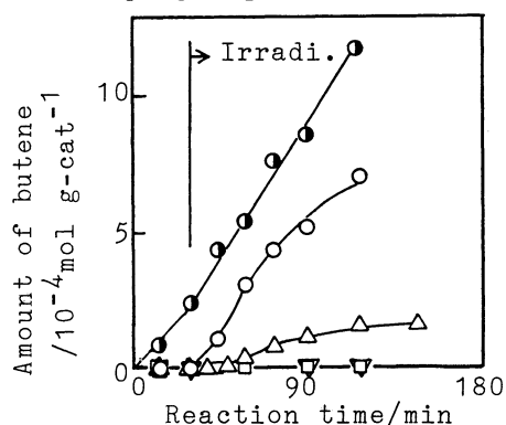
Fig. 1. Photoinduced metathesis on \text{Mo}(\text{CO})_6 /various supports. (●) \text{Al}_2\text{O}_3 , (○) \text{NaY} , (△) \text{PVG} , (□) \text{HY} , (▽) \text{TiO}_2 .
