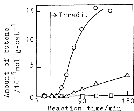
Fig. 2. Photoinduced metathesis on \text{Mo} , \text{W} , \text{Cr}(\text{CO})_6/\text{PVG} . (○) \text{Mo} , (△) \text{W} , (□) \text{Cr} .
